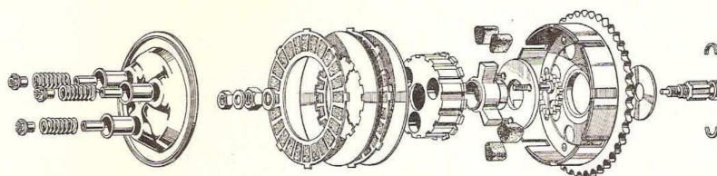
Fig. C31. Exploded View of Clutch.
