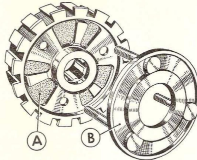
Fig. C32. Vane Assembly.
