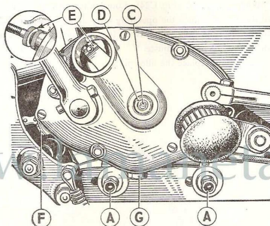
Fig. C24a. Clutch and Front Chain Adjustment.
