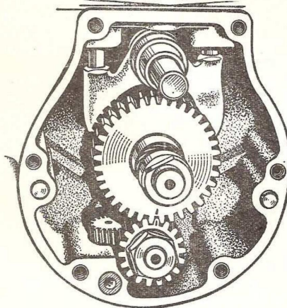
Fig. C.21. Valve-timing gears.
