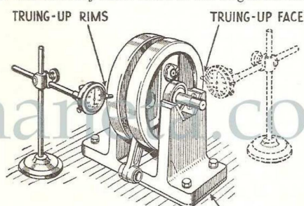
Suitable packing under timing side "vee" block to compensate for smaller diameter bearing. Fig. C.19. Checking flywheel alignment.
