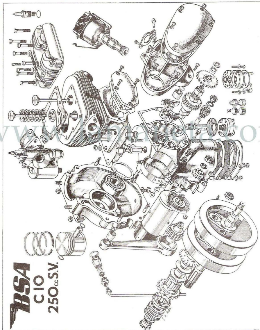
Fig. C1. The C10 Engine (Exploded View)
