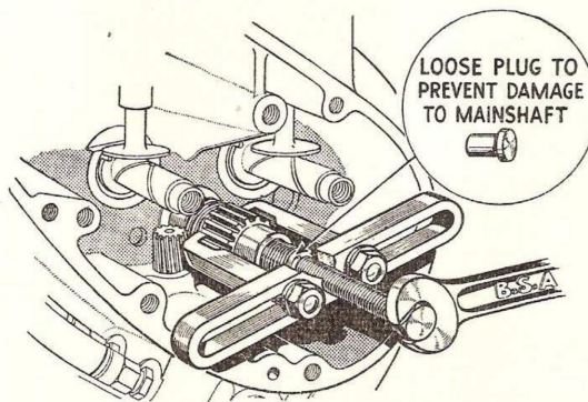
Fig. B.6. Engine Shaft Pinion Extractor 61-3256
