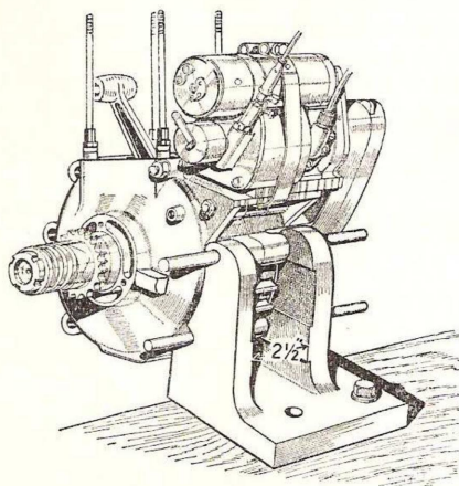
Fig. B.5. Angle Bracket for Mounting Engine
