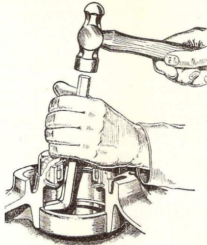
Fig. B.8. Roller-race extraction (driveside).
