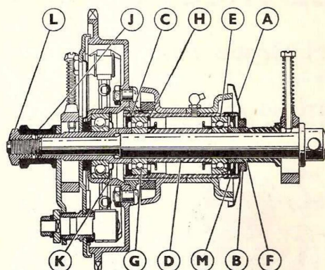
Fig. A32(c). Section through the Rear Hub
