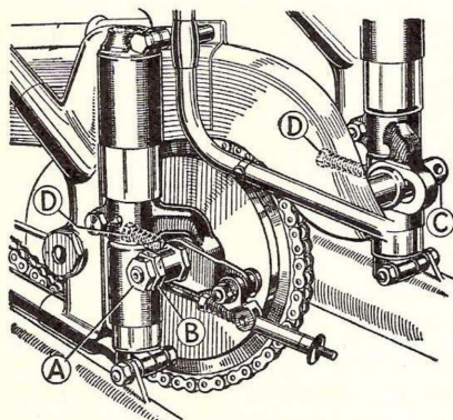
Fig. A33(c). Rear Chain Adjustment
