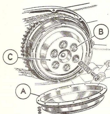
Fig. A26. Clutch spring adjustment.
