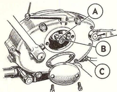
Fig. A25. Clutch control adjustment.
