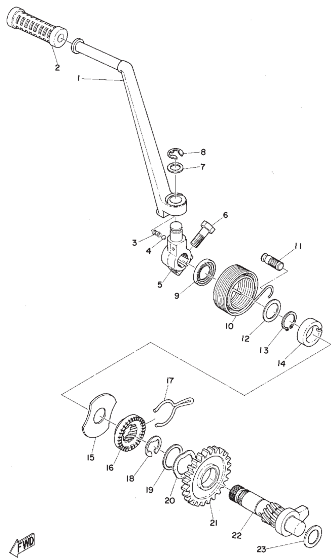
Fig. 9 KICK STARTER
