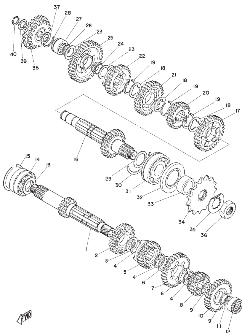
Fig. 6 TRANSMISSION
