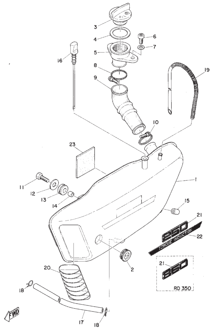
Fig. 27 OIL TANK
