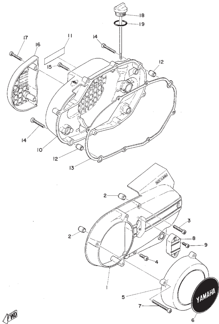
Fig. 3 CRANKCASE COVER
