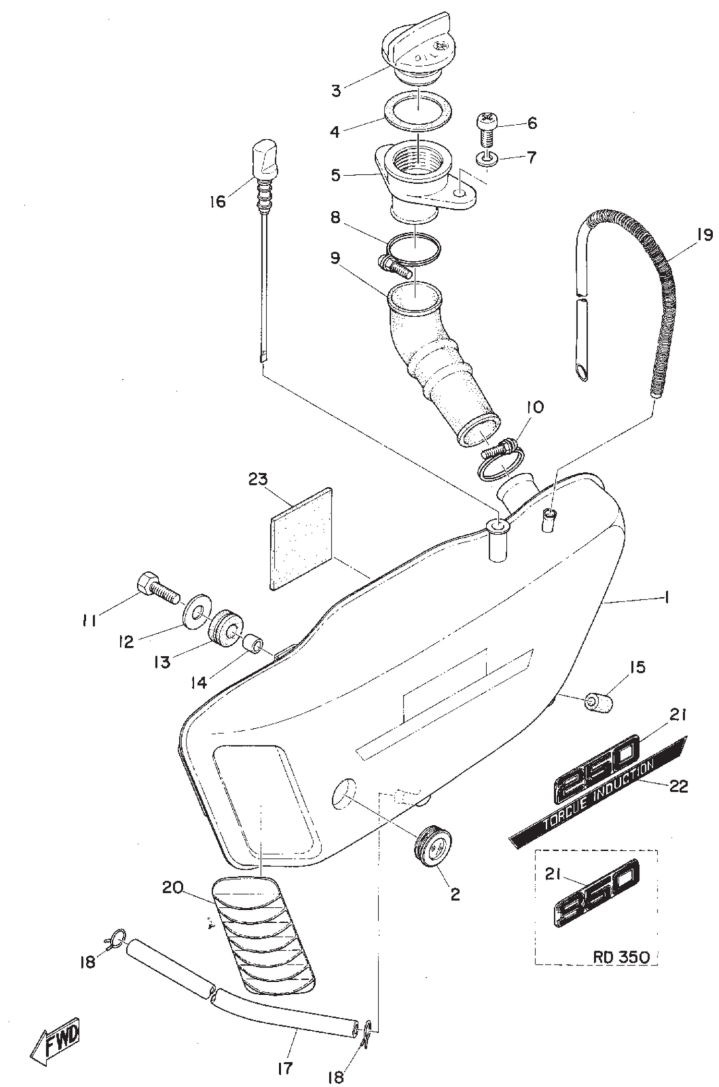
Fig. 27 OIL TANK
