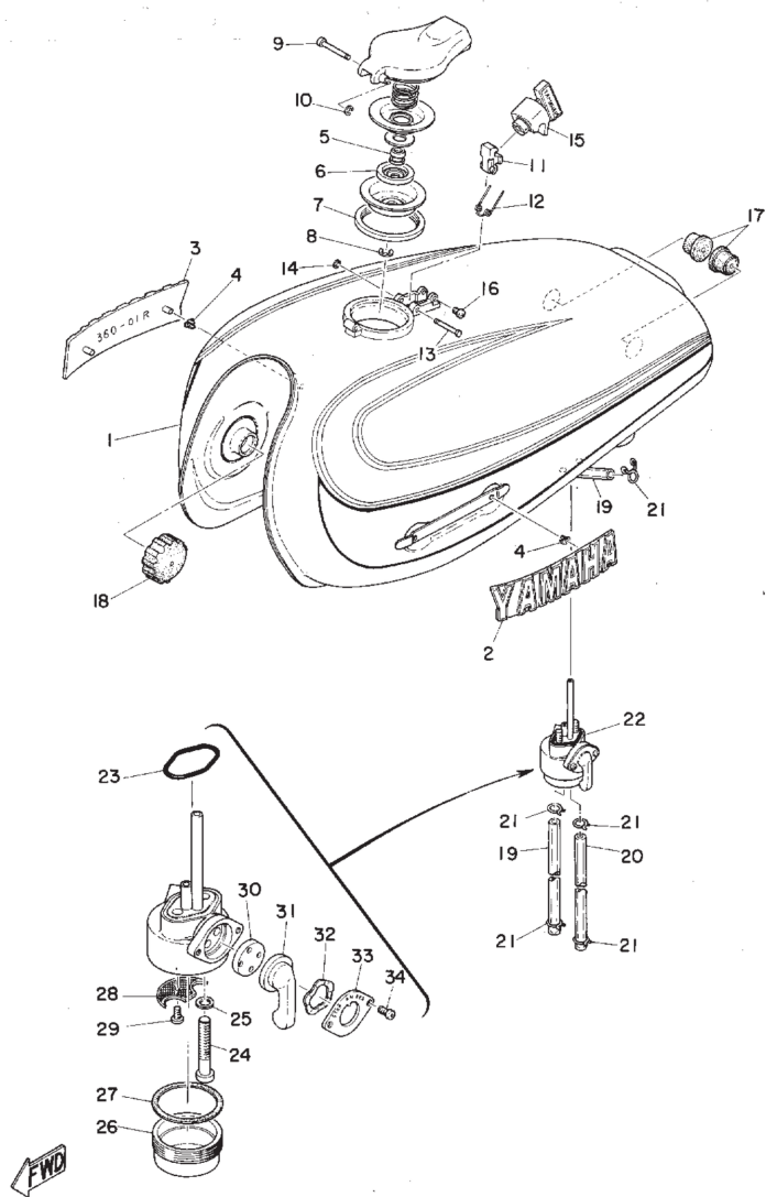
Fig. 26 FUEL TANK
