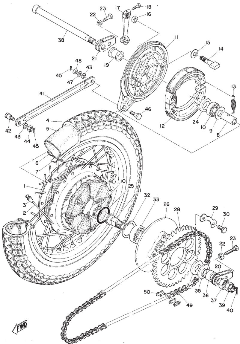
Fig. 32 REAR WHEEL
