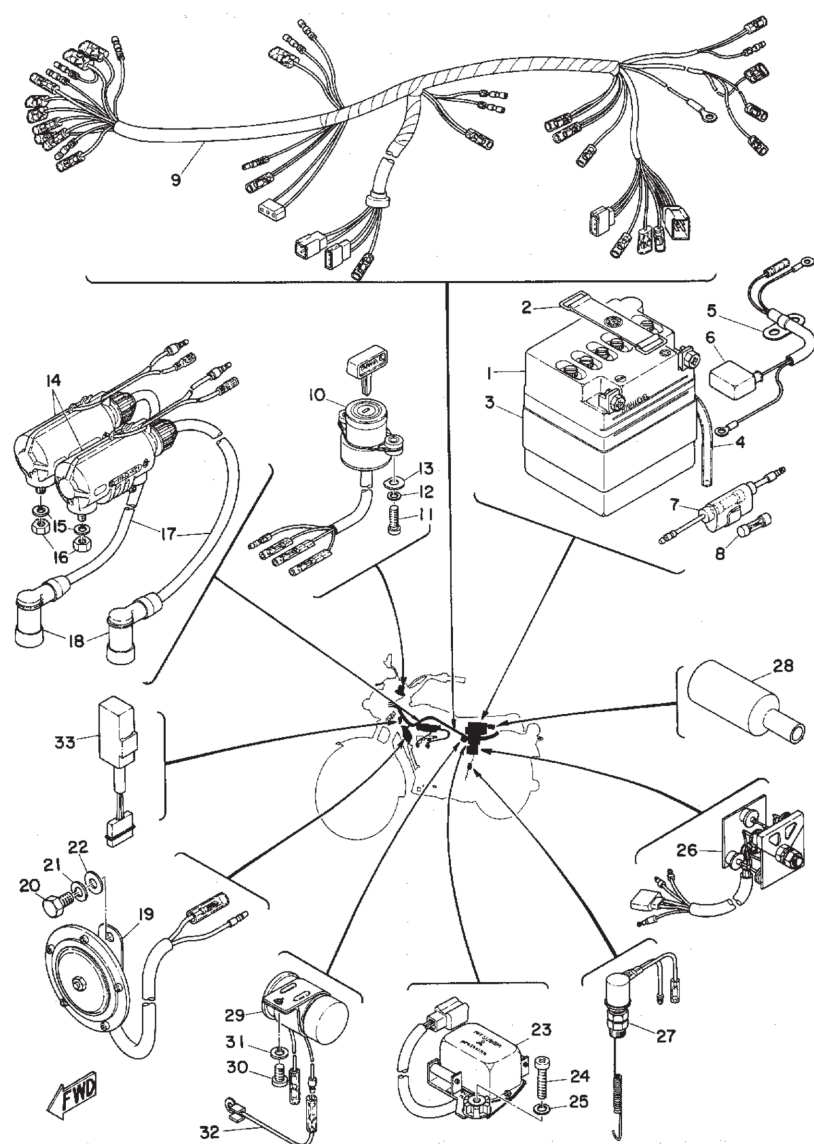
Fig. 37 ELECTRICAL
