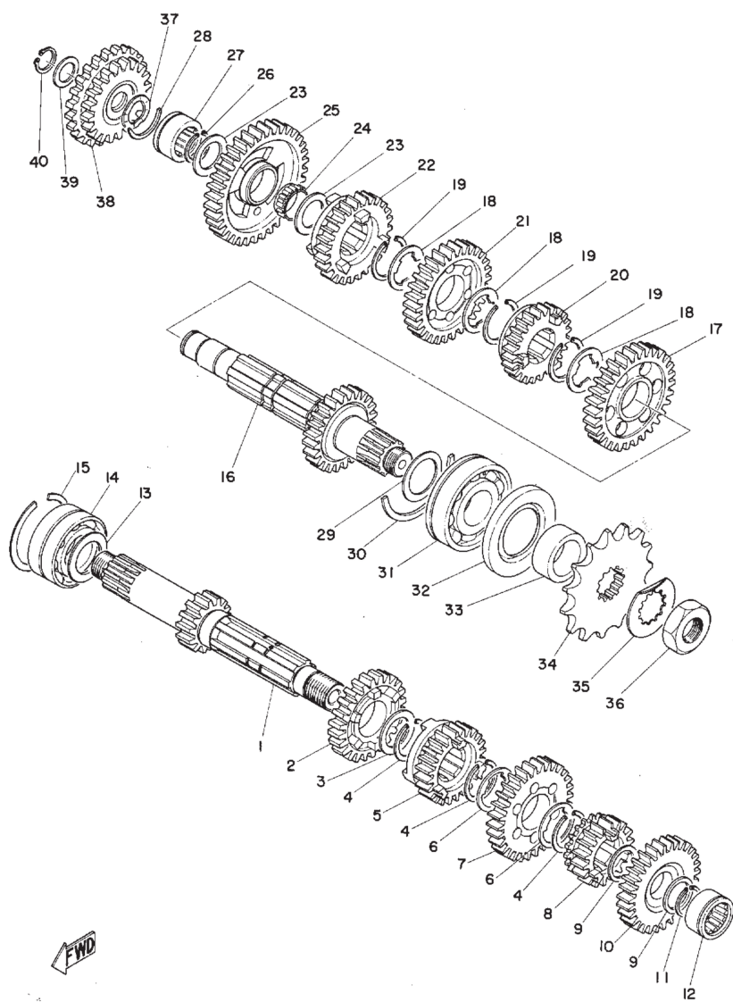
Fig. 6 TRANSMISSION
