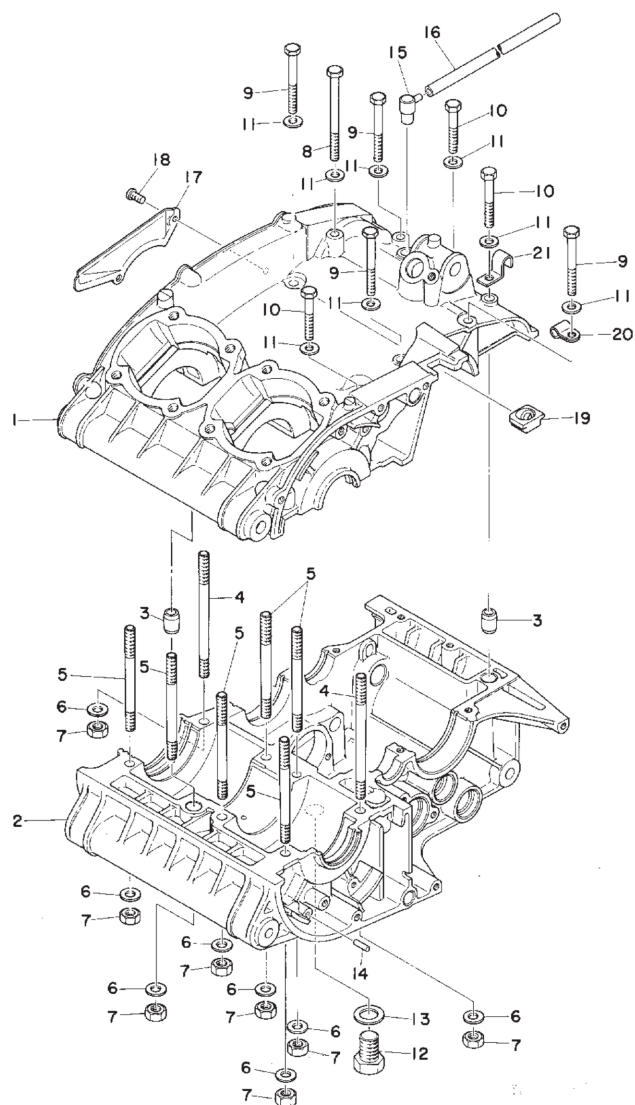
Fig. 2 CRANKCASE
